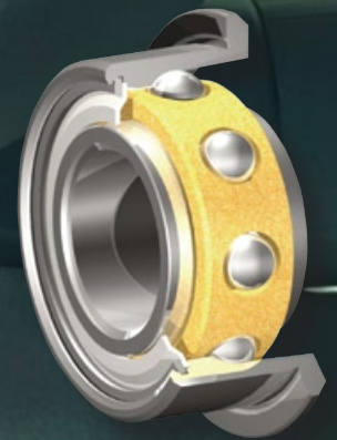
Angular Contact Single Shield (Machined Full Type)
